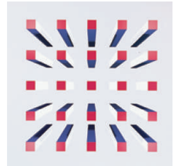
Figure 37.14 Computer simulation of the appearance of an array of 25 rods with square cross section. The center rod is viewed end-on. The simulation ignores color changes in the array caused by the Doppler effect (see Section 37.6).
